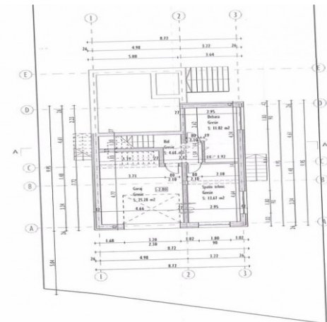
PLAN SUBSOL SCARA 1:100
