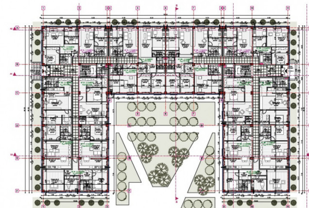
PLAN PARTER
