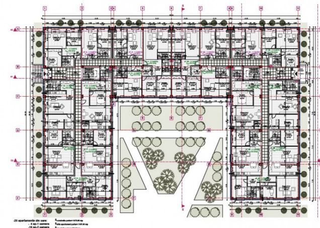
PLAN PARTER
